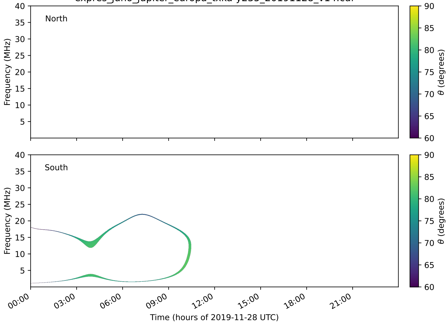
expres_juno_jupiter_europa_txka-y235_20191128_v14.cdf
