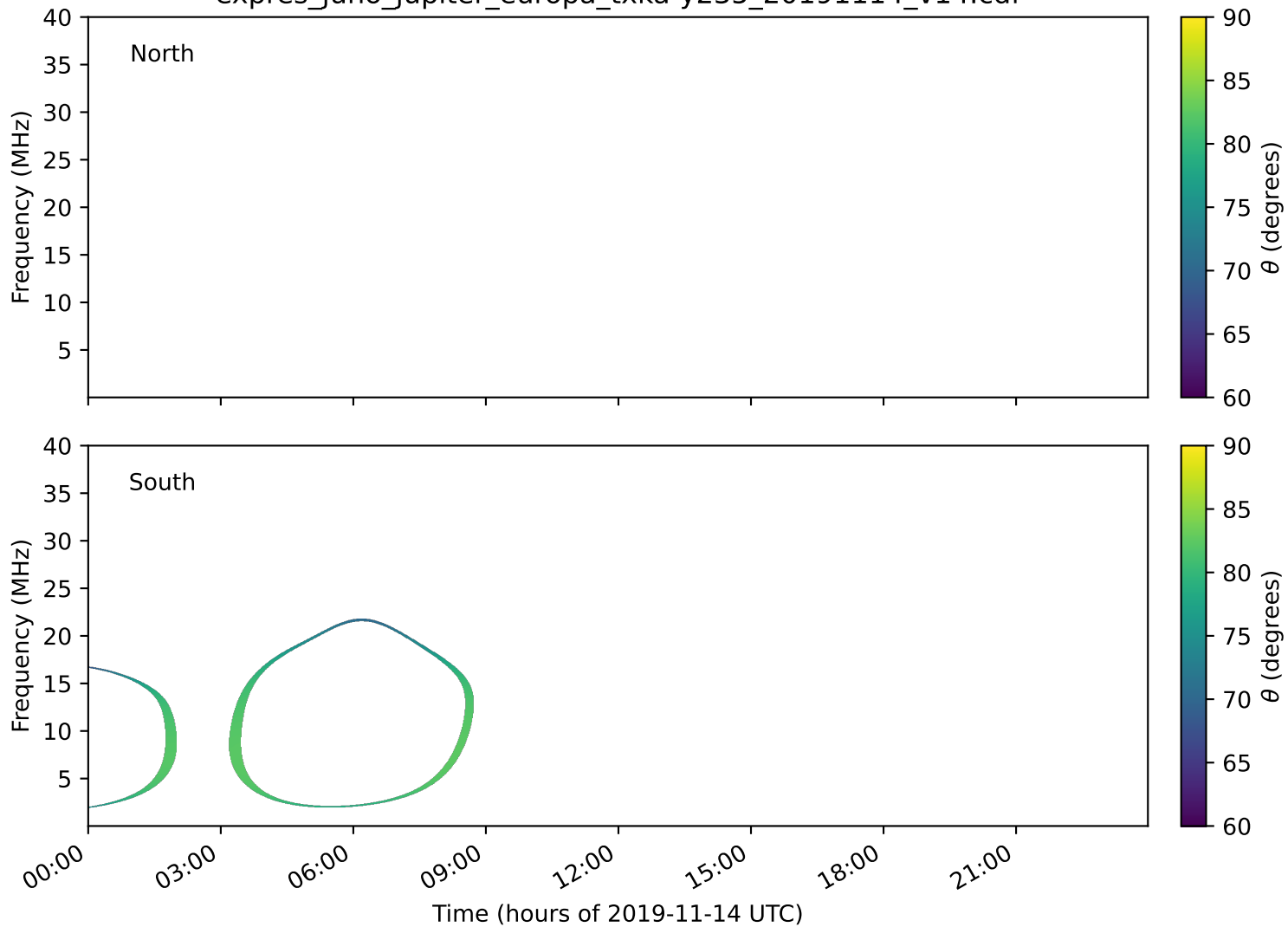
expres_juno_jupiter_europa_txka-y235_20191114_v14.cdf
