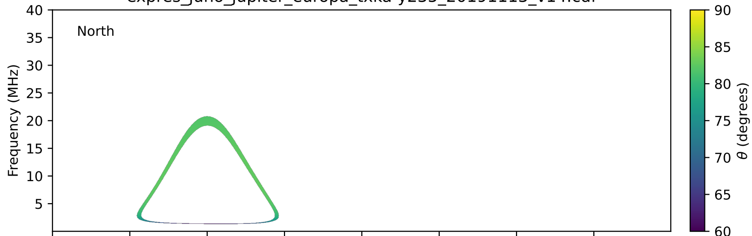
expres_juno_jupiter_europa_txka-y235_20191113_v14.cdf
