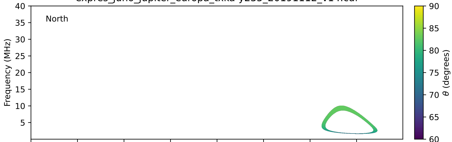
expres_juno_jupiter_europa_txka-y235_20191112_v14.cdf
