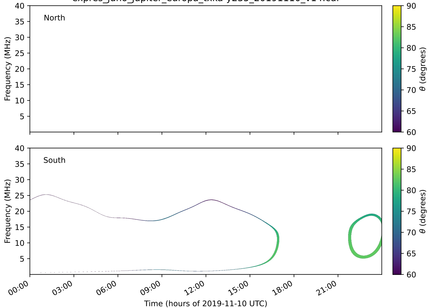
expres_juno_jupiter_europa_txka-y235_20191110_v14.cdf
