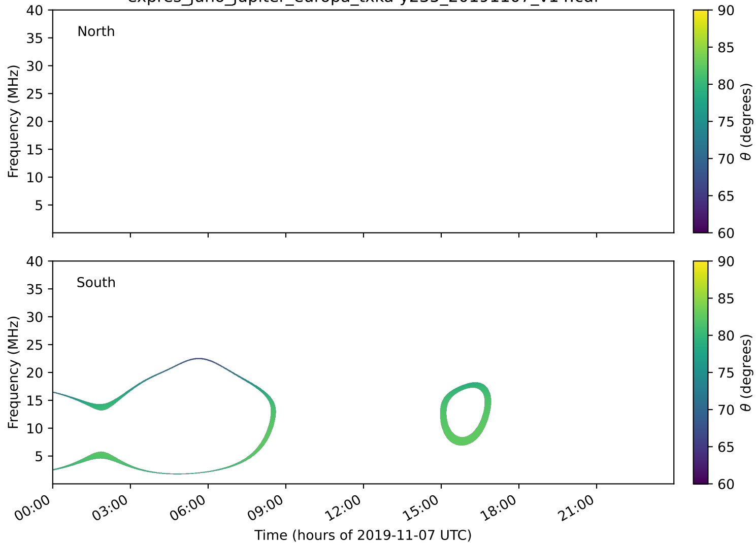
expres_juno_jupiter_europa_txka-y235_20191107_v14.cdf
