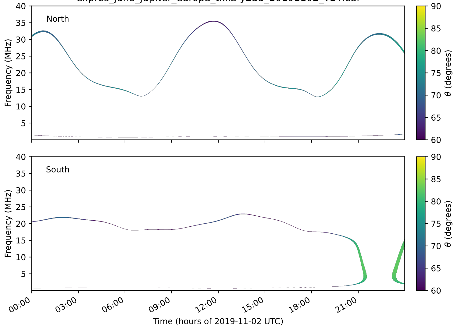
expres_juno_jupiter_europa_txka-y235_20191102_v14.cdf
