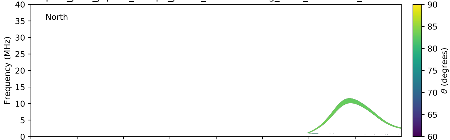
expres_juno_jupiter_europa_jrm09_lossc-wid1deg_3kev_20191119_v01.cdf
