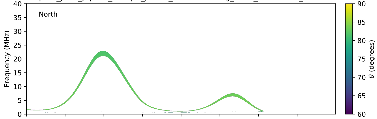
expres_juno_jupiter_europa_jrm09_lossc-wid1deg_3kev_20191113_v01.cdf
