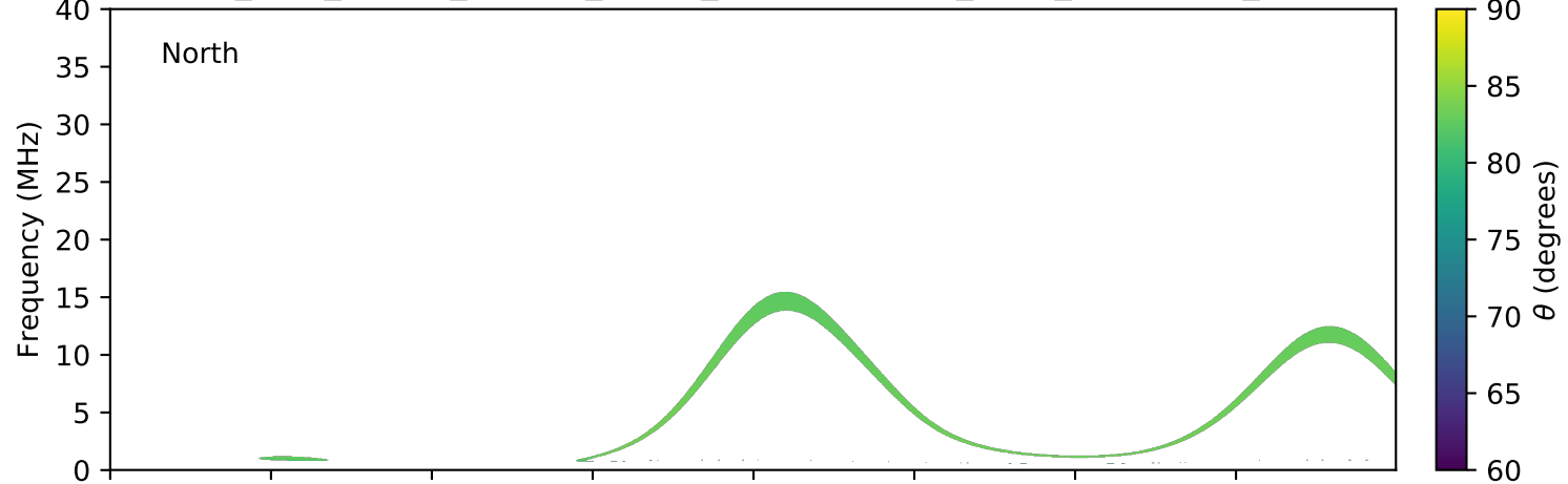
expres_juno_jupiter_europa_jrm09_lossc-wid1deg_3kev_20191109_v01.cdf
