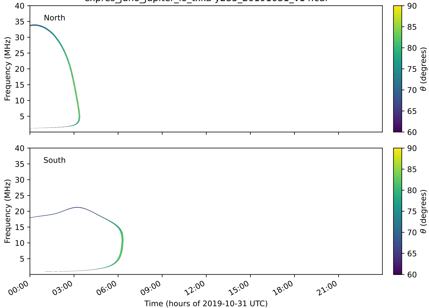
expres_juno_jupiter_io_txka-y235_20191031_v14.cdf
