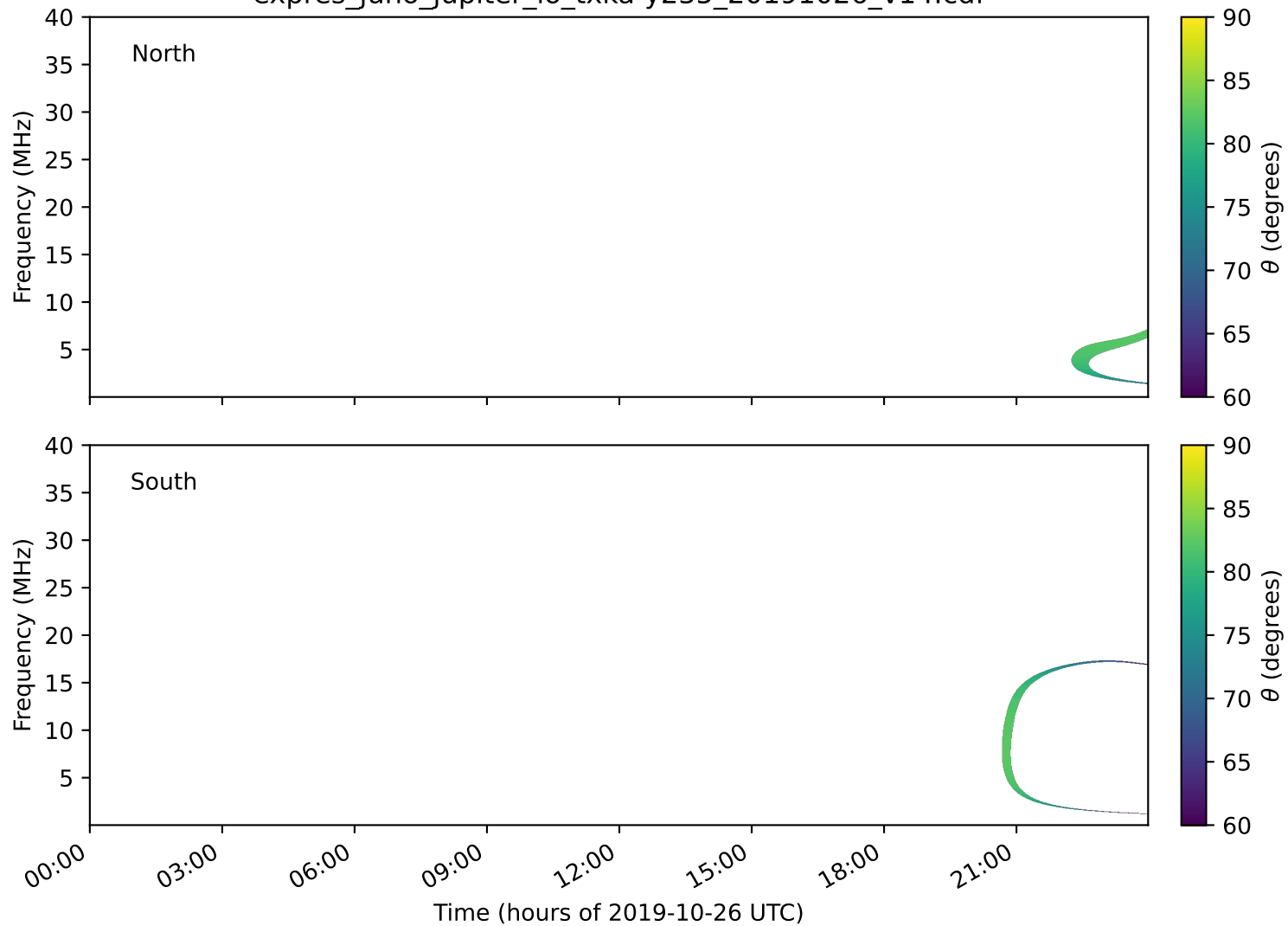
expres_juno_jupiter_io_txka-y235_20191026_v14.cdf
