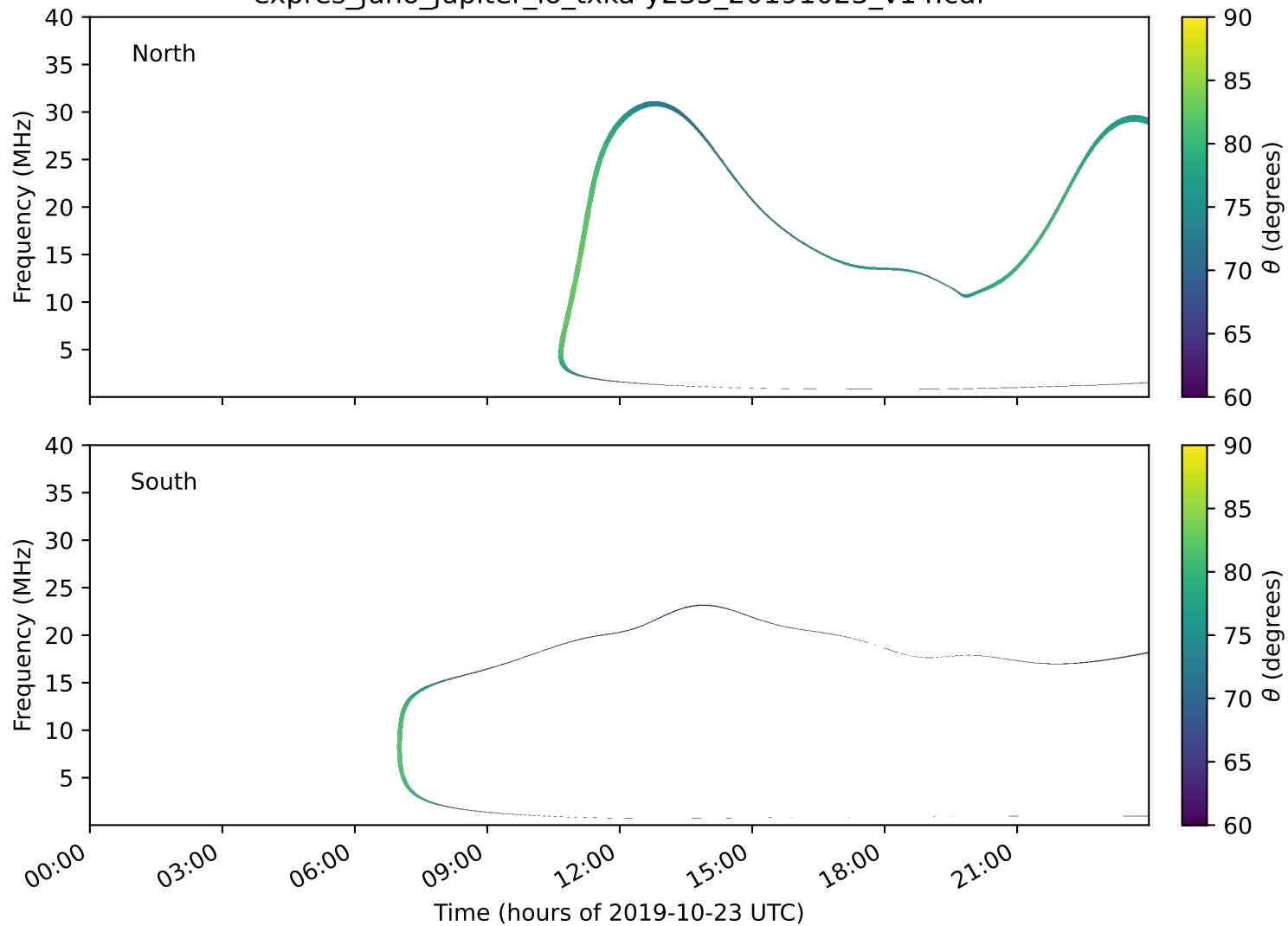
expres_juno_jupiter_io_txka-y235_20191023_v14.cdf
