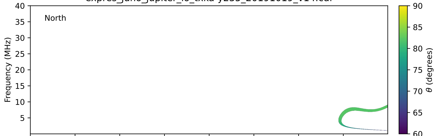
expres_juno_jupiter_io_txka-y235_20191019_v14.cdf
