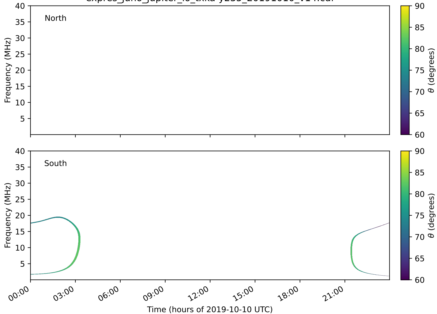
expres_juno_jupiter_io_txka-y235_20191010_v14.cdf
