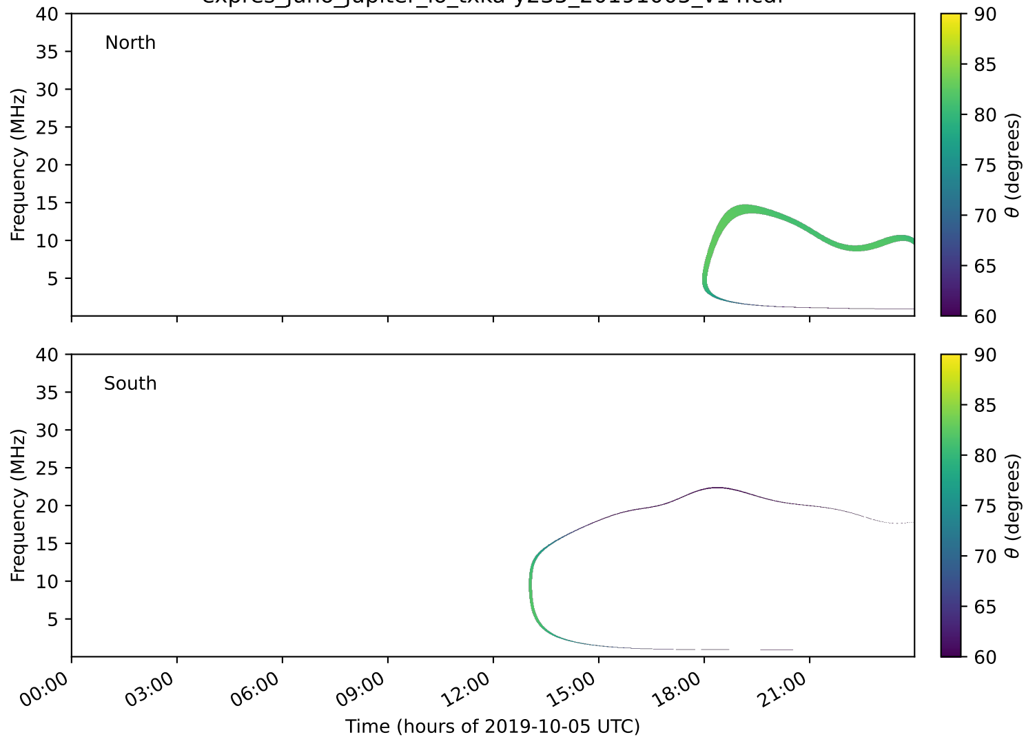
expres_juno_jupiter_io_txka-y235_20191005_v14.cdf
