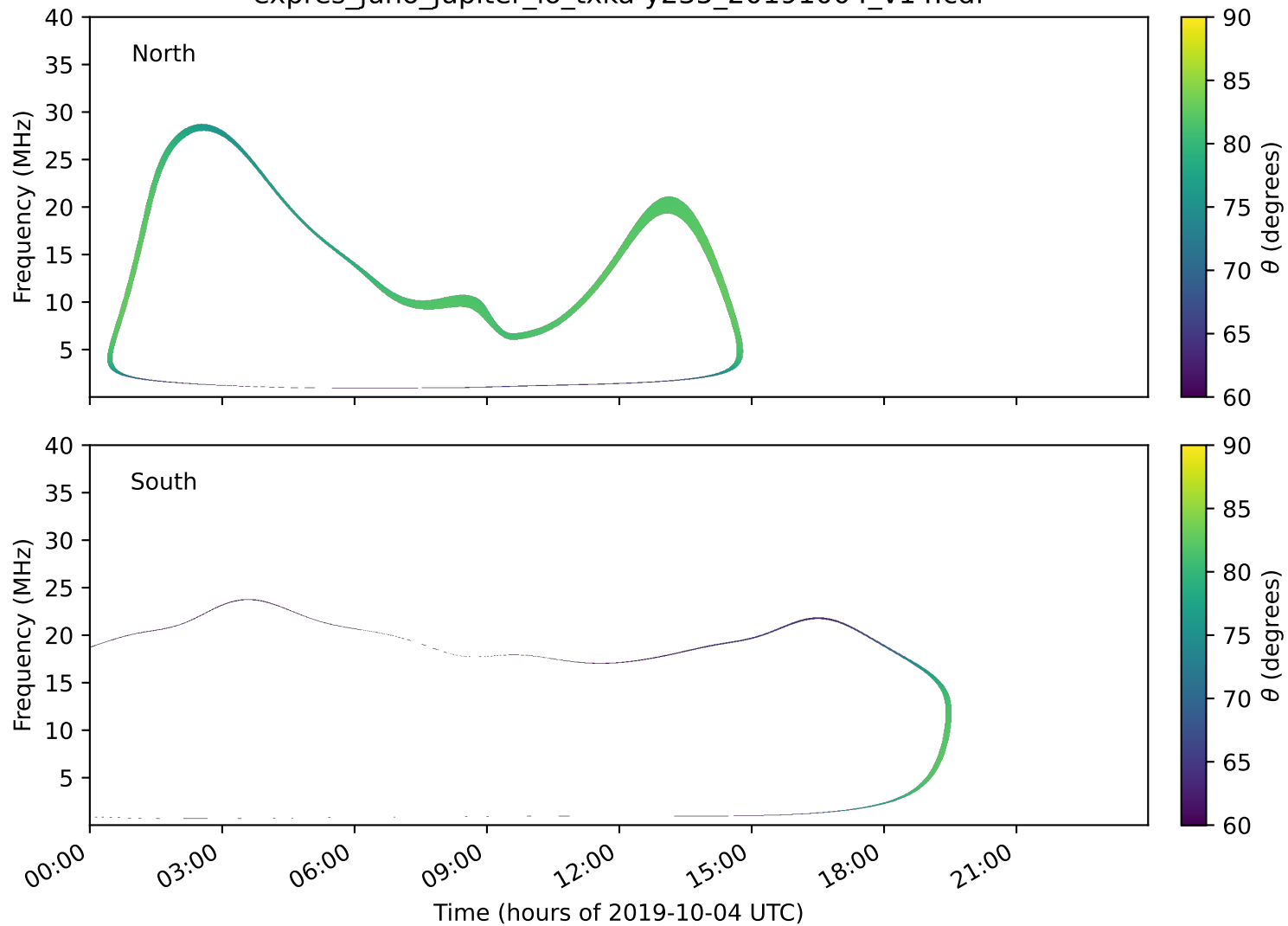
expres_juno_jupiter_io_txka-y235_20191004_v14.cdf
