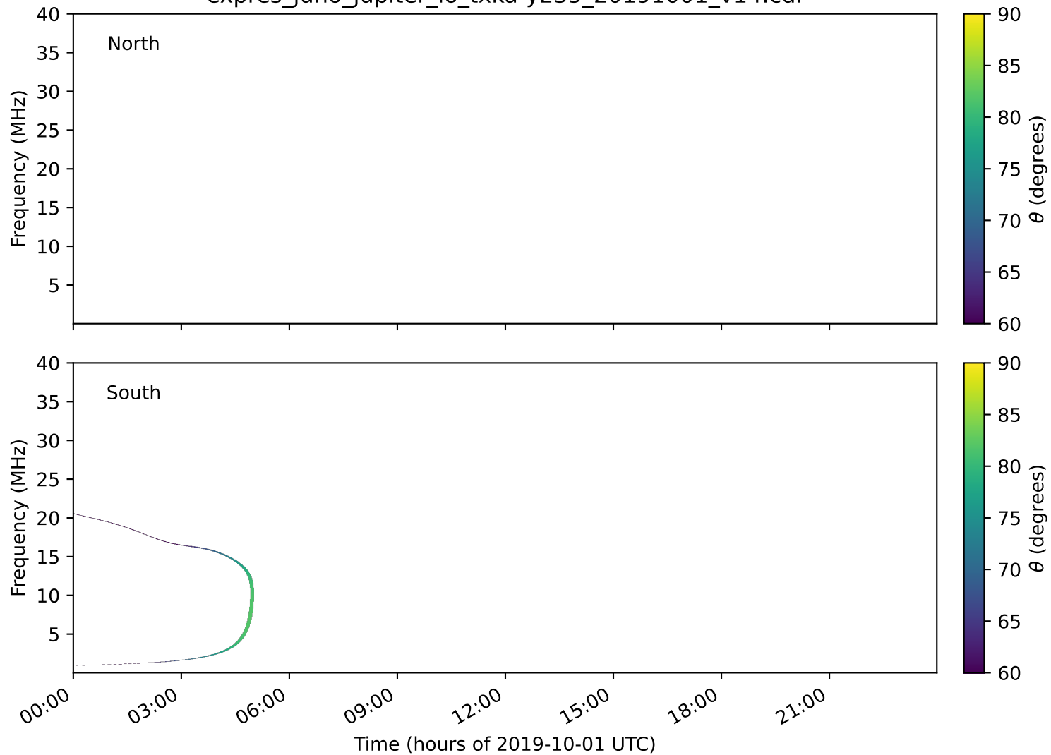
expres_juno_jupiter_io_txka-y235_20191001_v14.cdf
