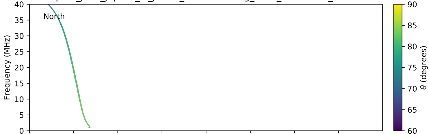
expres_juno_jupiter_io_jrm09_lossc-wid1deg_3kev_20191031_v01.cdf
