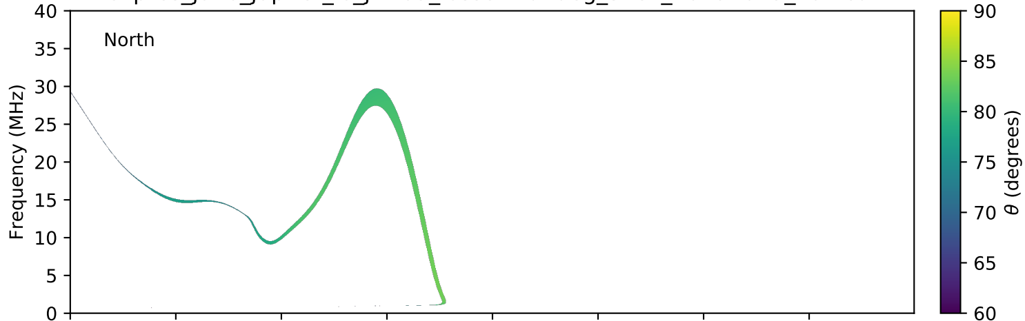
expres_juno_jupiter_io_jrm09_lossc-wid1deg_3kev_20191029_v01.cdf
