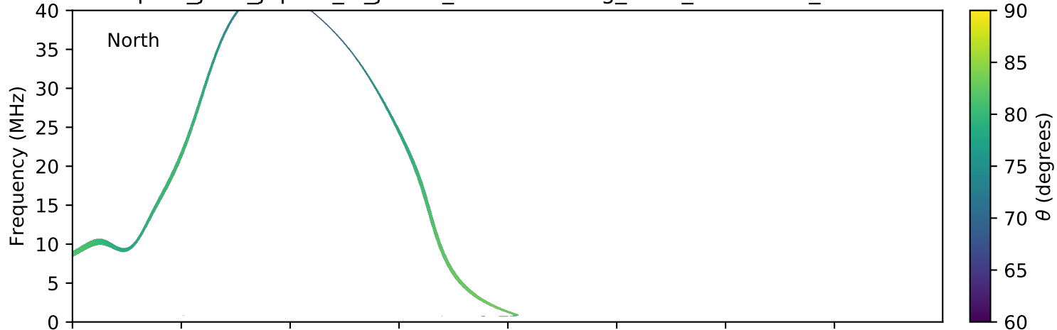
expres_juno_jupiter_io_jrm09_lossc-wid1deg_3kev_20191020_v01.cdf
