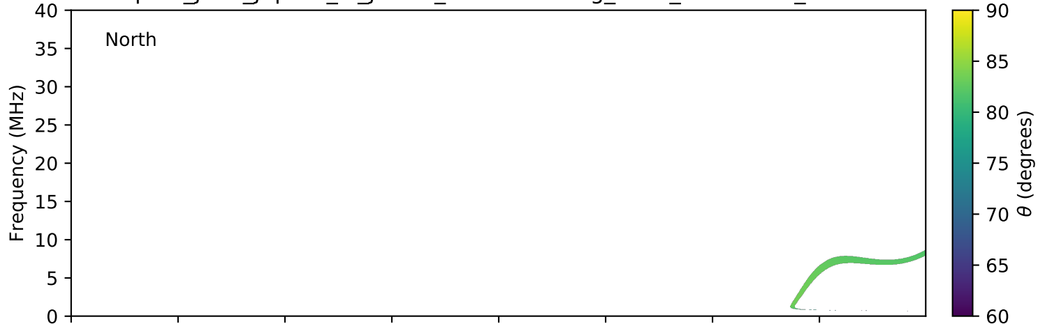
expres_juno_jupiter_io_jrm09_lossc-wid1deg_3kev_20191019_v01.cdf
