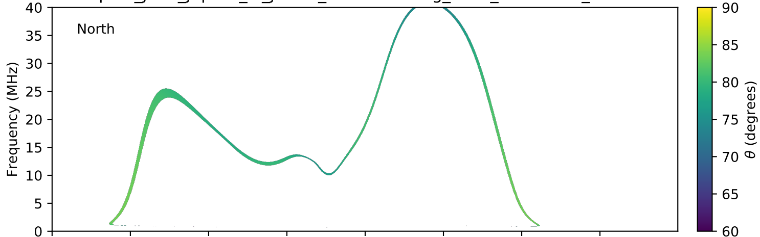
expres_juno_jupiter_io_jrm09_lossc-wid1deg_3kev_20191018_v01.cdf
