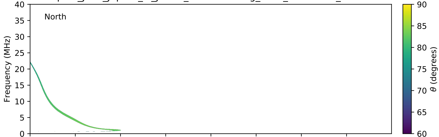
expres_juno_jupiter_io_jrm09_lossc-wid1deg_3kev_20191015_v01.cdf
