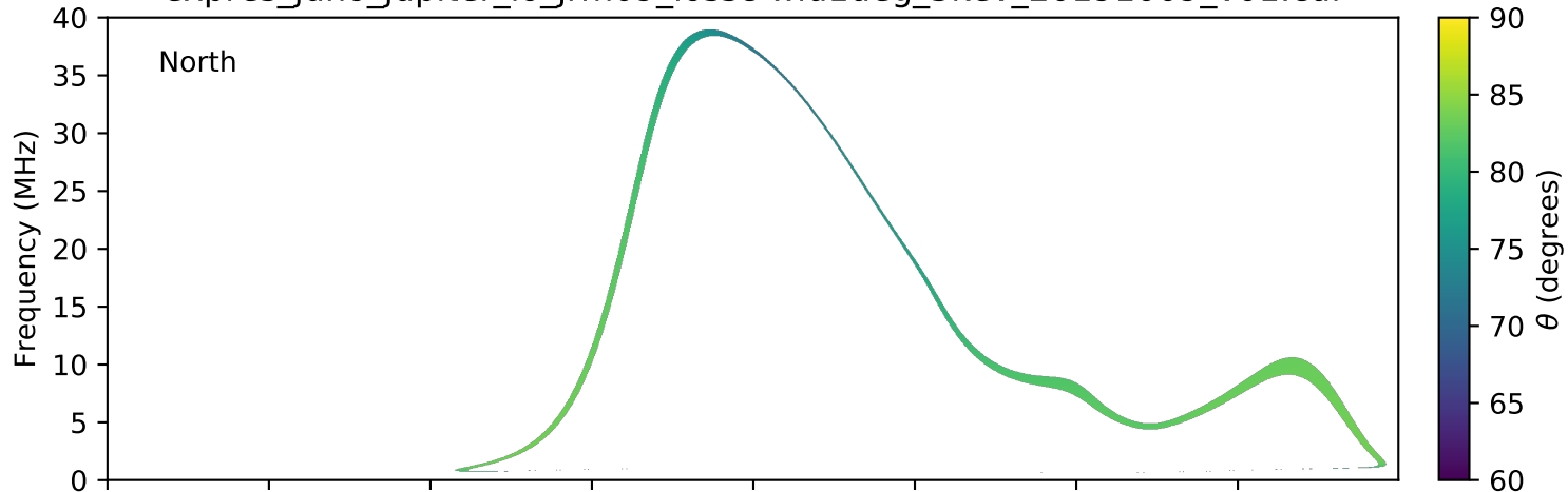
expres_juno_jupiter_io_jrm09_lossc-wid1deg_3kev_20191009_v01.cdf
