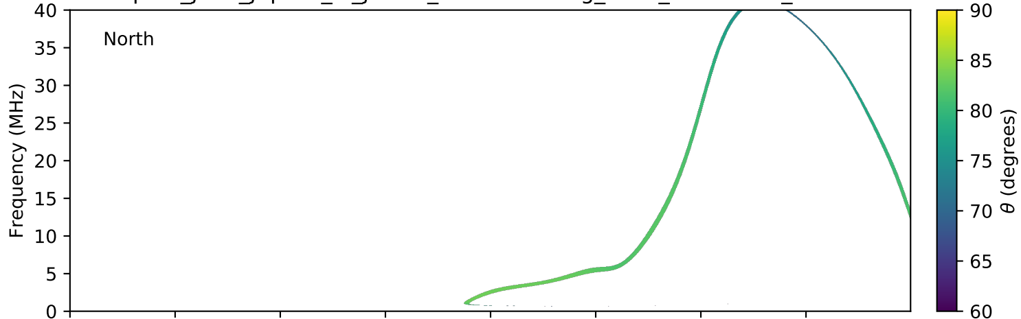
expres_juno_jupiter_io_jrm09_lossc-wid1deg_3kev_20191007_v01.cdf
