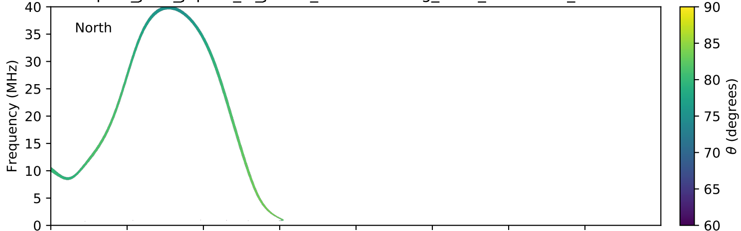
expres_juno_jupiter_io_jrm09_lossc-wid1deg_3kev_20191006_v01.cdf
