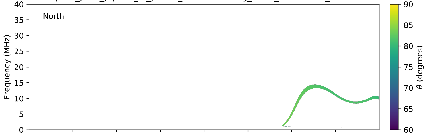
expres_juno_jupiter_io_jrm09_lossc-wid1deg_3kev_20191005_v01.cdf
