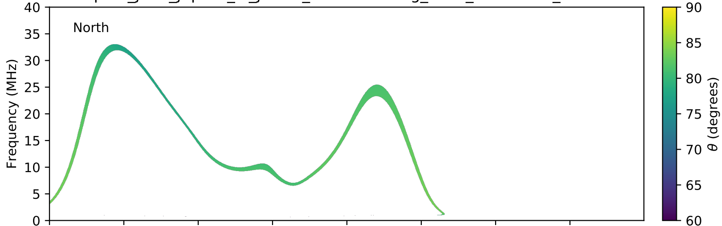
expres_juno_jupiter_io_jrm09_lossc-wid1deg_3kev_20191004_v01.cdf
