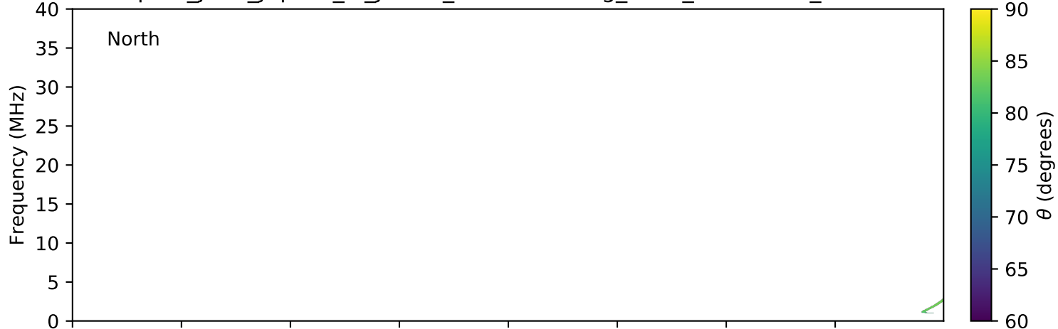
expres_juno_jupiter_io_jrm09_lossc-wid1deg_3kev_20191003_v01.cdf
