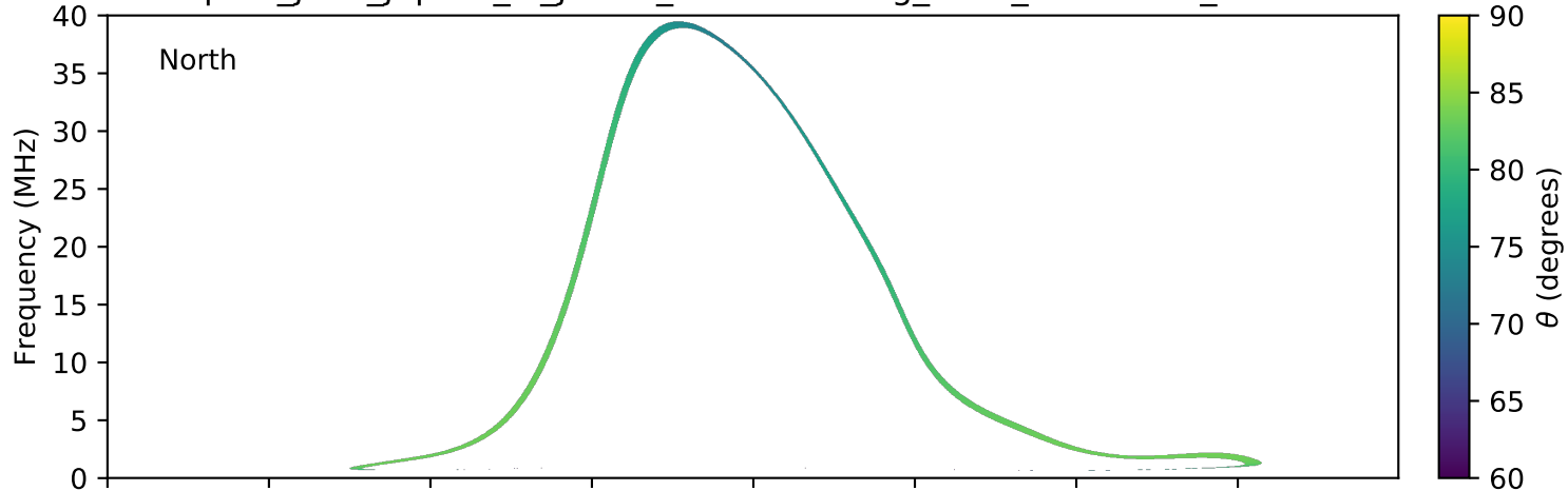
expres_juno_jupiter_io_jrm09_lossc-wid1deg_3kev_20191002_v01.cdf
