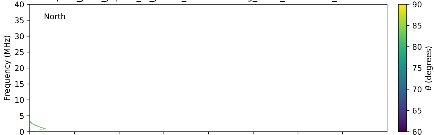
expres_juno_jupiter_io_jrm09_lossc-wid1deg_3kev_20191001_v01.cdf
