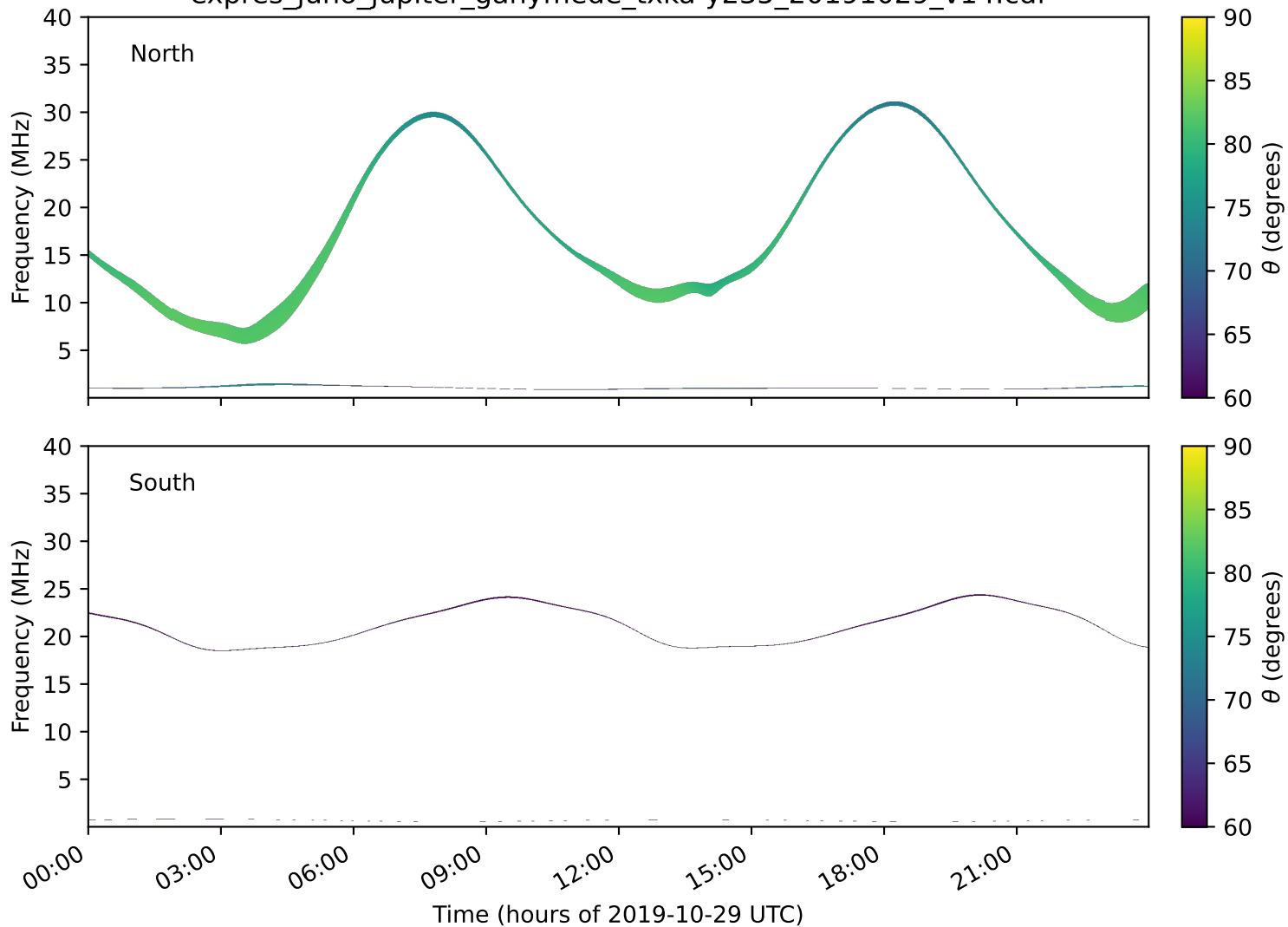
expres_juno_jupiter_ganymede_txka-y235_20191029_v14.cdf
