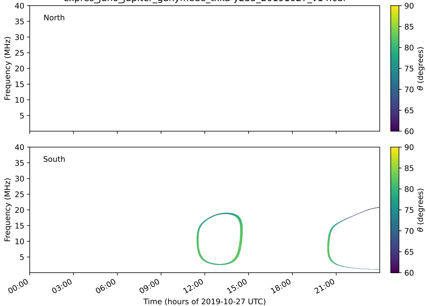
expres_juno_jupiter_ganymede_txka-y235_20191027_v14.cdf
