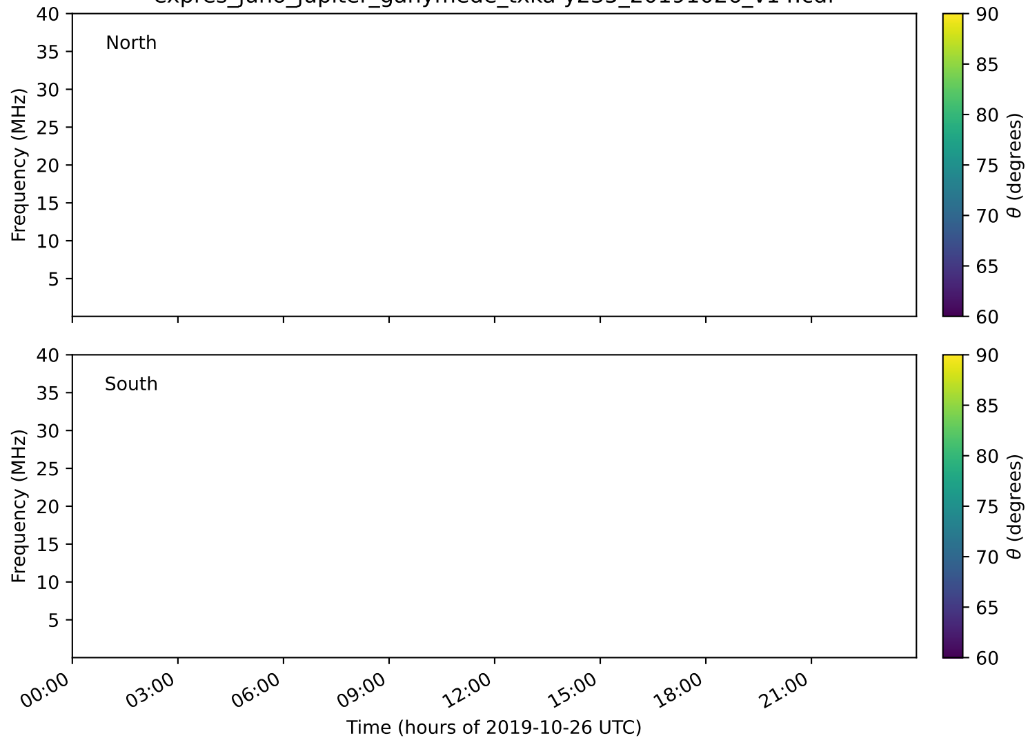
expres_juno_jupiter_ganymede_txka-y235_20191026_v14.cdf
