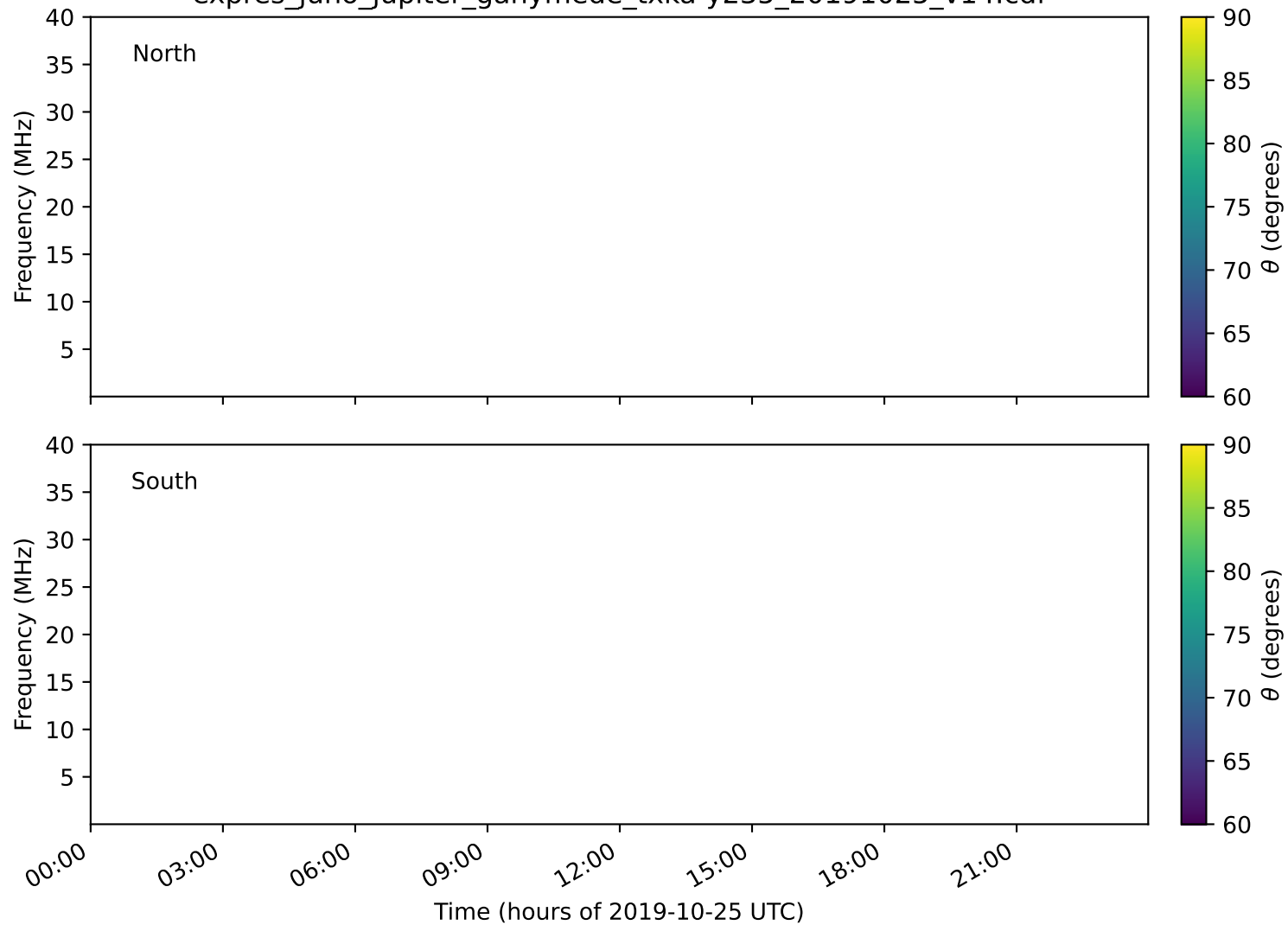
expres_juno_jupiter_ganymede_txka-y235_20191025_v14.cdf
