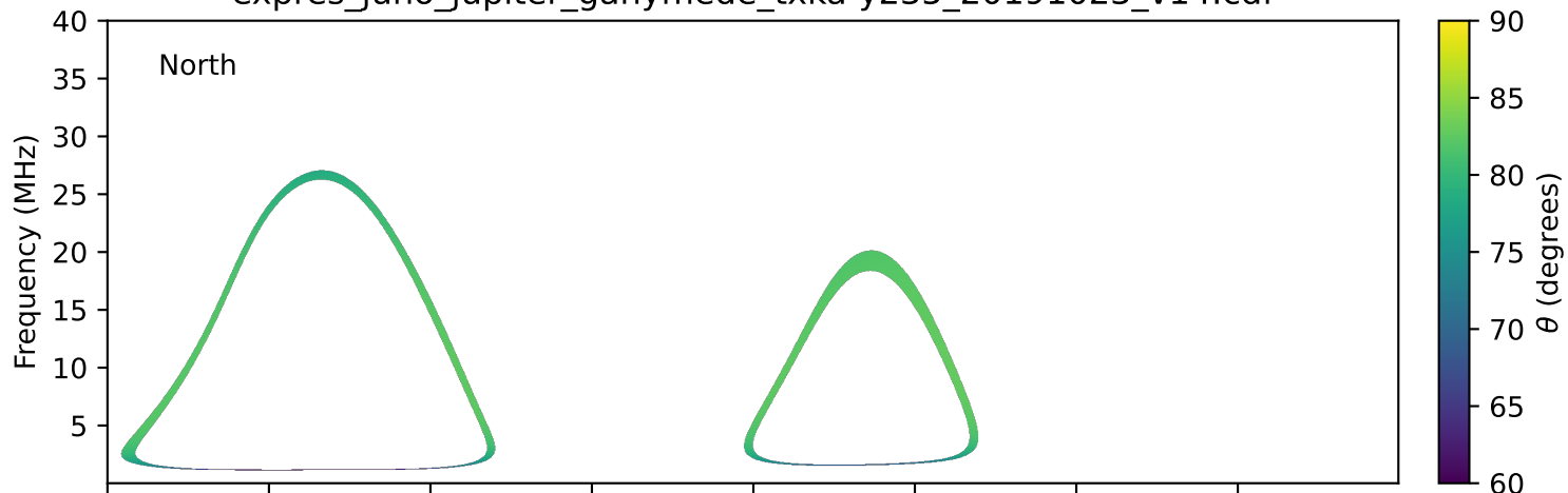
expres_juno_jupiter_ganymede_txka-y235_20191023_v14.cdf
