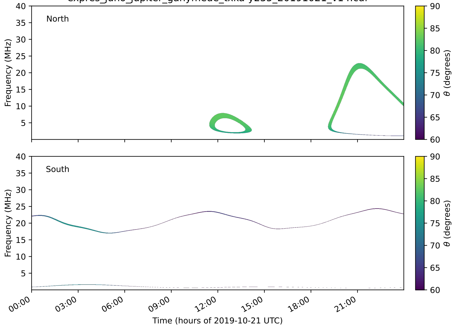
expres_juno_jupiter_ganymede_txka-y235_20191021_v14.cdf
