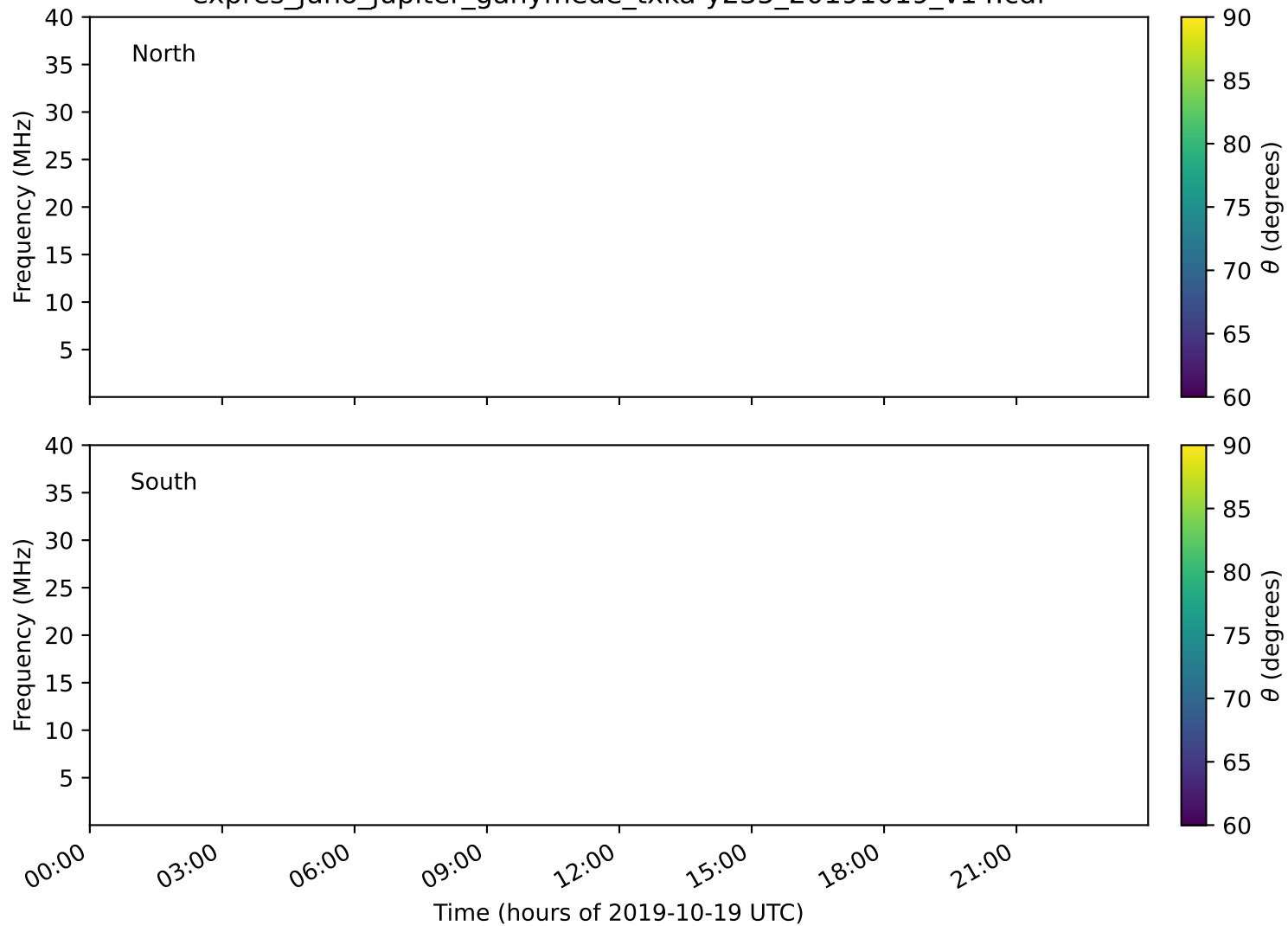
expres_juno_jupiter_ganymede_txka-y235_20191019_v14.cdf
