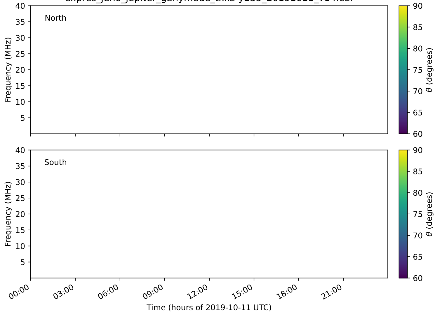
expres_juno_jupiter_ganymede_txka-y235_20191011_v14.cdf
