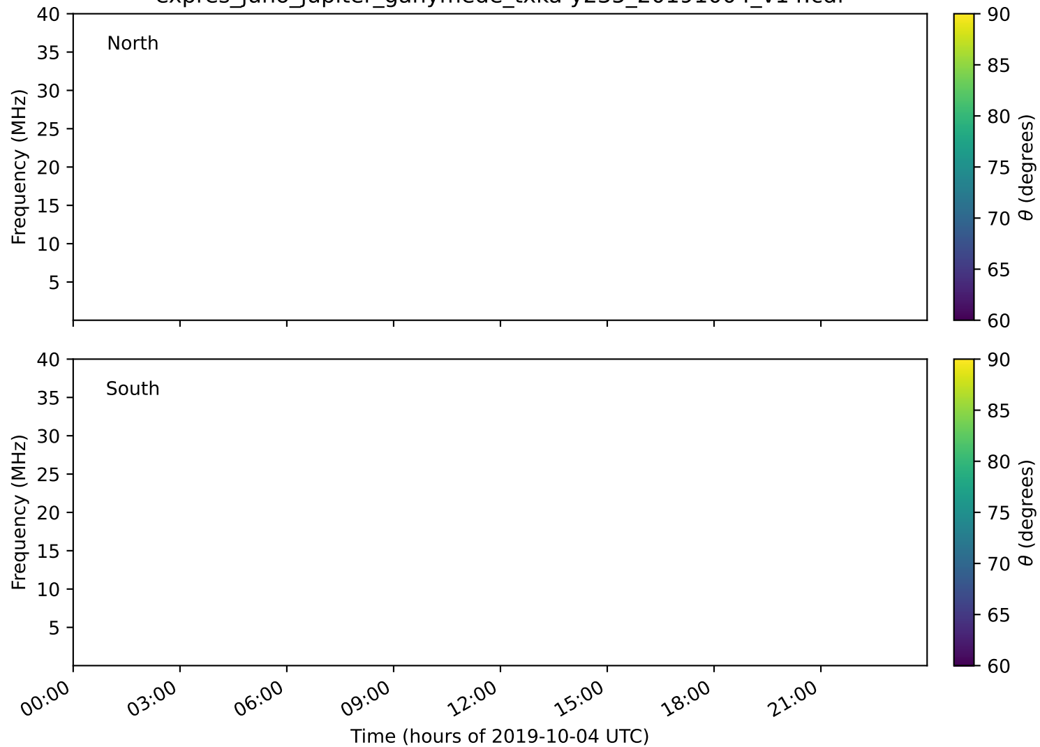
expres_juno_jupiter_ganymede_txka-y235_20191004_v14.cdf
