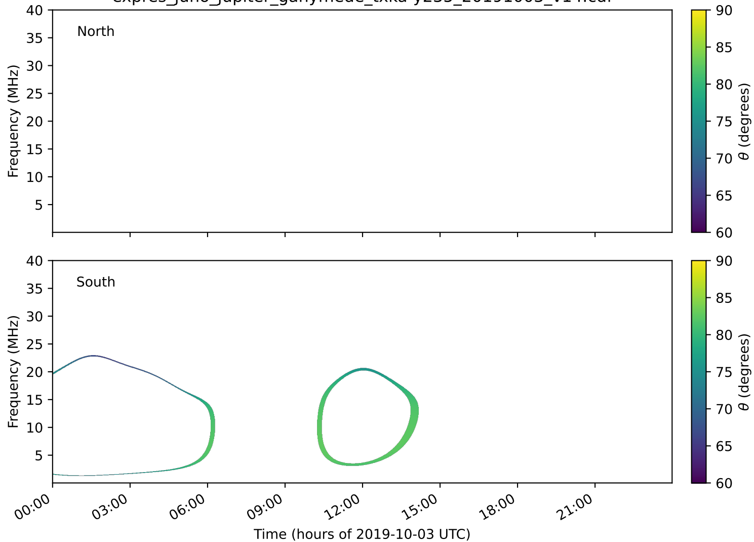
expres_juno_jupiter_ganymede_txka-y235_20191003_v14.cdf
