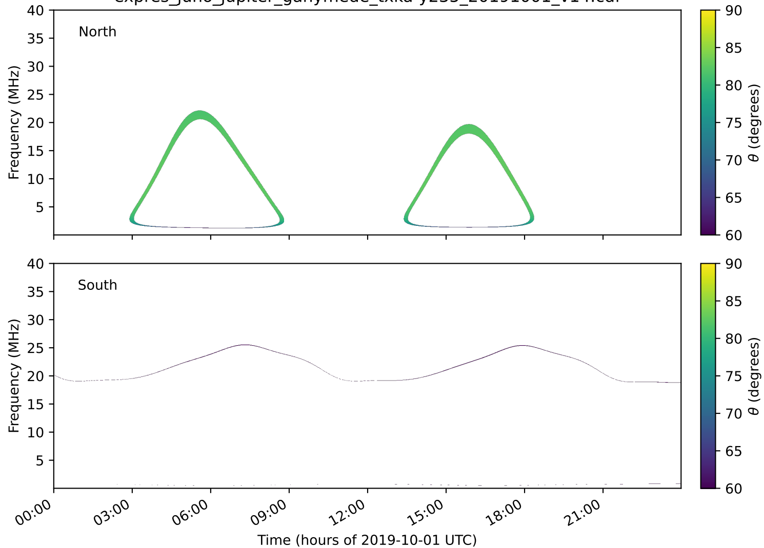
expres_juno_jupiter_ganymede_txka-y235_20191001_v14.cdf
