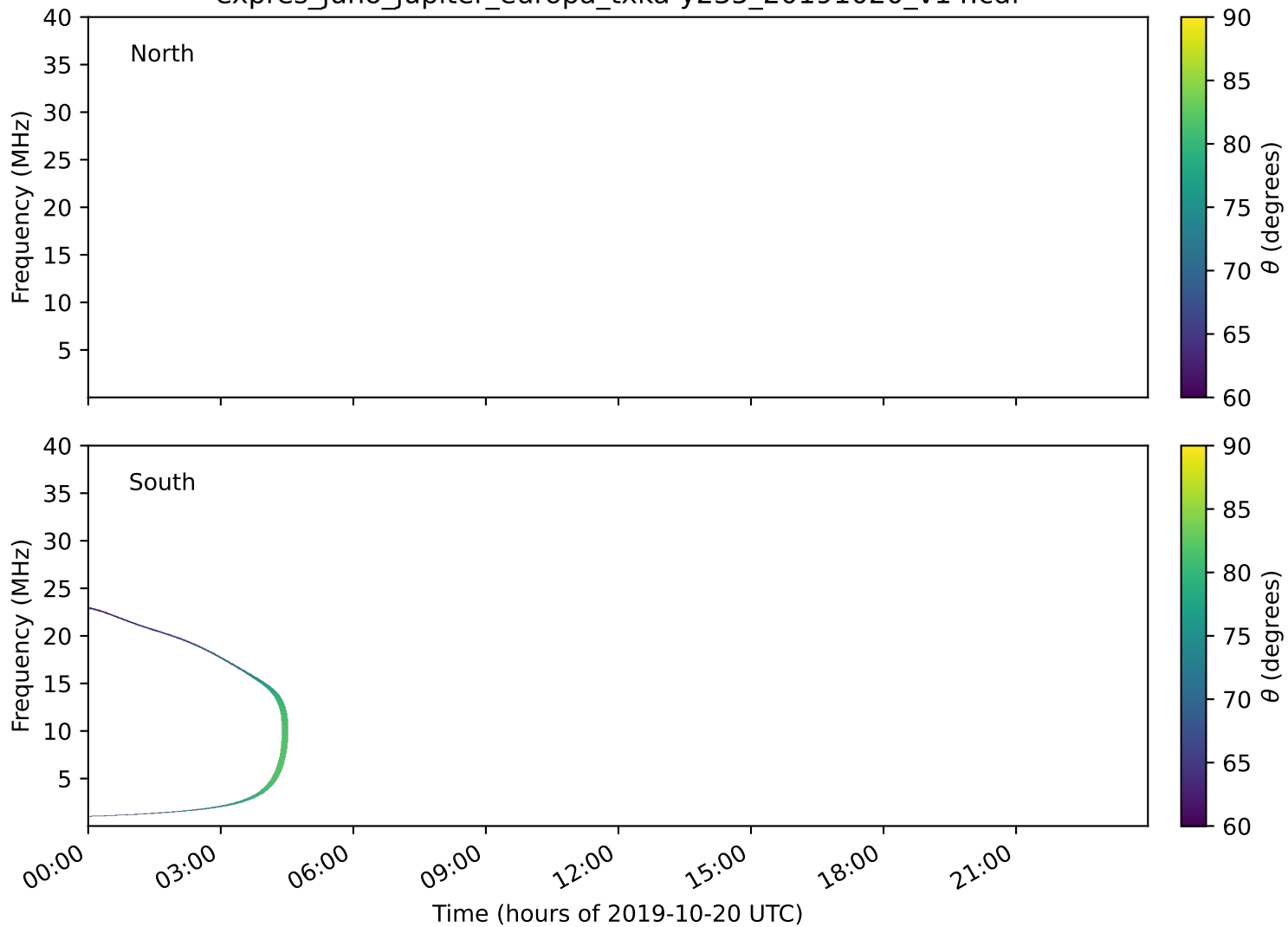
expres_juno_jupiter_europa_txka-y235_20191020_v14.cdf
