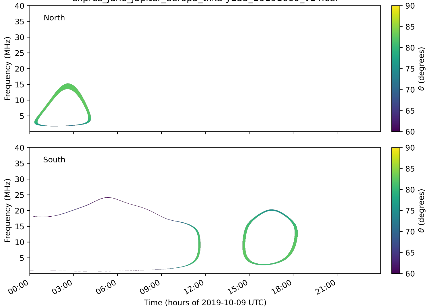
expres_juno_jupiter_europa_txka-y235_20191009_v14.cdf
