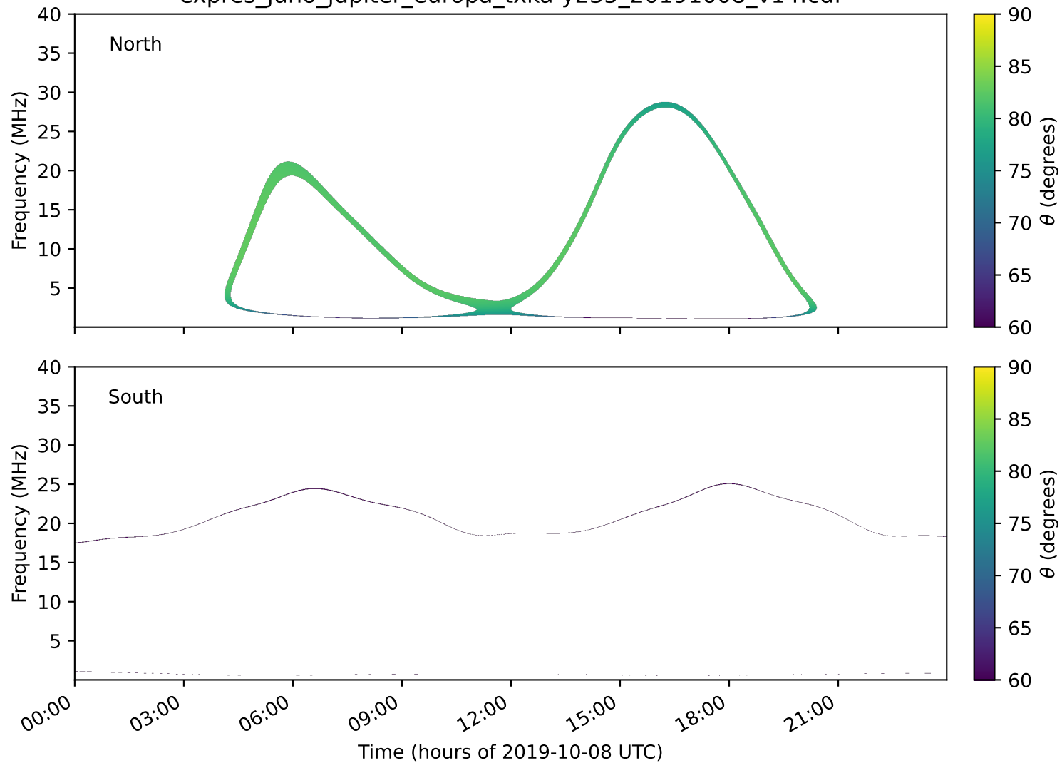
expres_juno_jupiter_europa_txka-y235_20191008_v14.cdf
