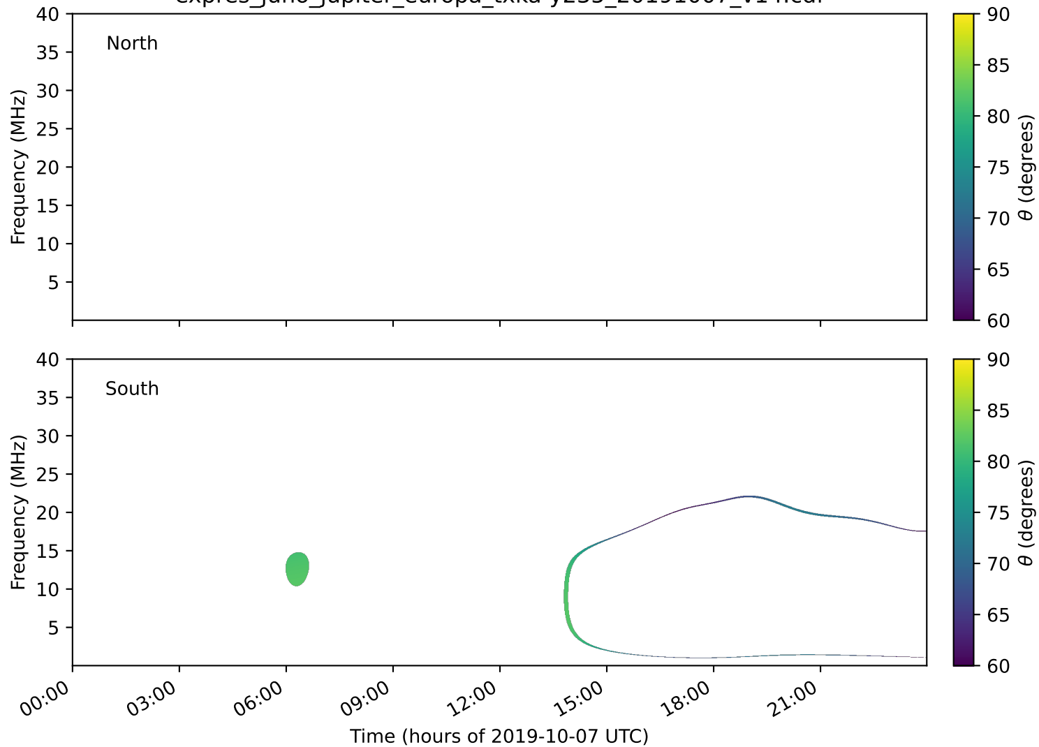
expres_juno_jupiter_europa_txka-y235_20191007_v14.cdf
