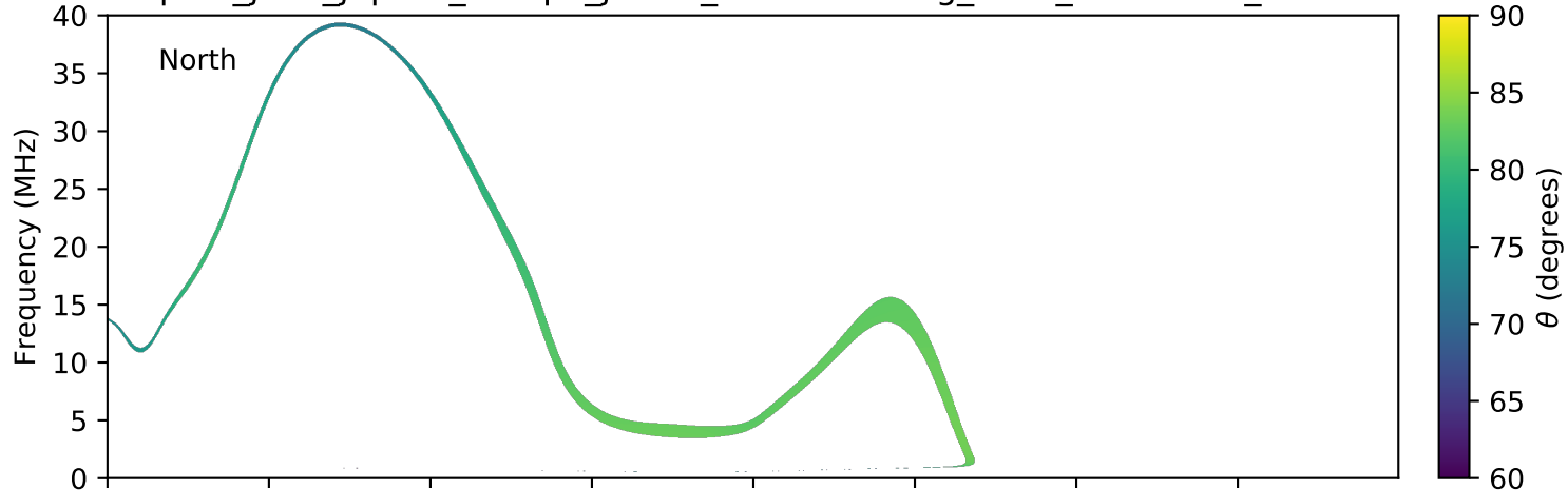
expres_juno_jupiter_europa_jrm09_lossc-wid1deg_3kev_20191030_v01.cdf
