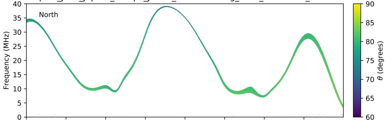
expres_juno_jupiter_europa_jrm09_lossc-wid1deg_3kev_20191026_v01.cdf
