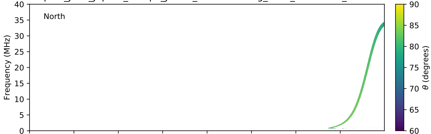
expres_juno_jupiter_europa_jrm09_lossc-wid1deg_3kev_20191025_v01.cdf
